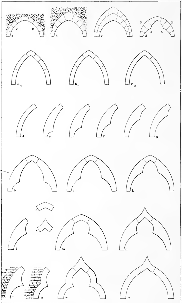
PLATE III.—ARCH MASONRY.
